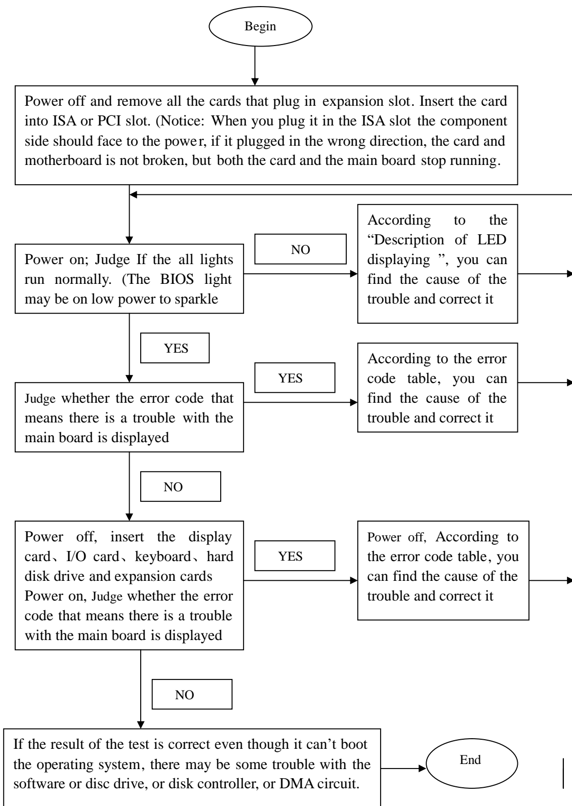
Illustration of four-bit code POST card (5004 version)
